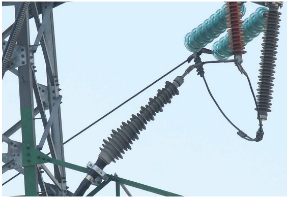
Dry type outdoor termination angle mounted on a tower.
