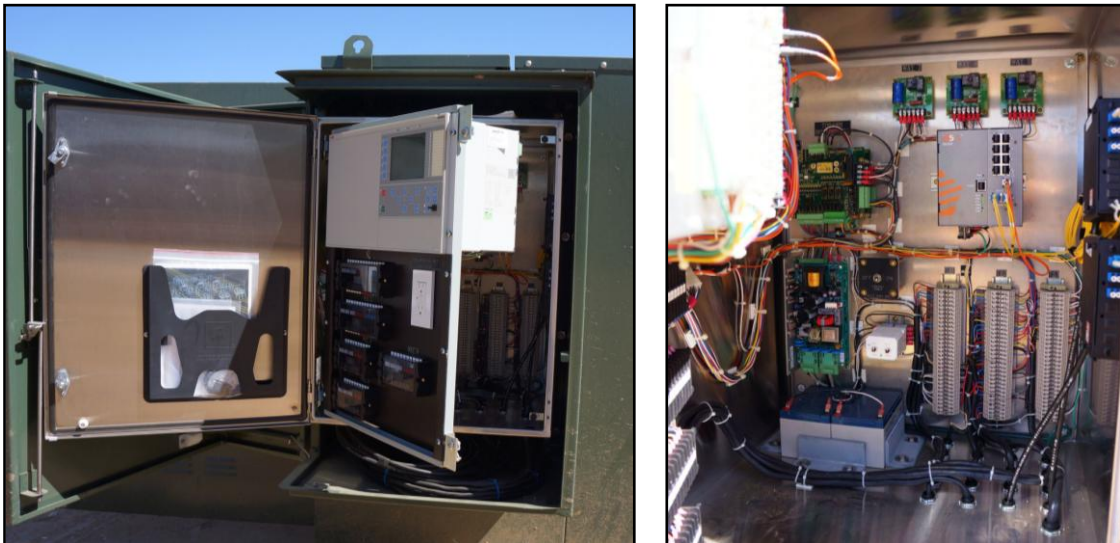
Figure 8: Switch control cabinet with relay, test switches, Ethernet switch, and batteries
